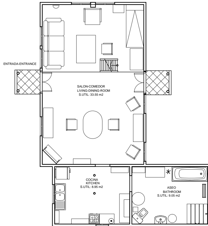
PLANTA BAJA GROUND FLOOR
