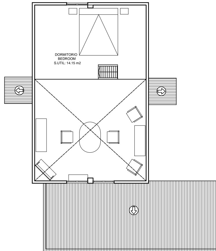
PLANTA ALTA UPSTAIRS
